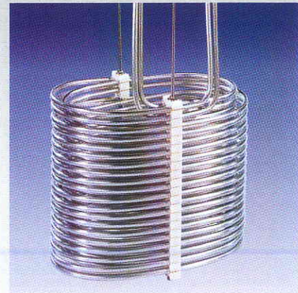
Basket evaporator
