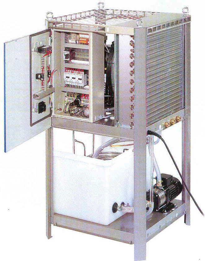
Basket evaporator
